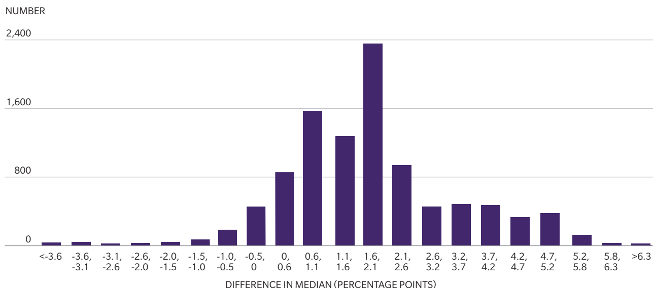
Figure 52: Median Difference of Baseline Gender Balance Definition Histogram from Bootstrapped Simulations
