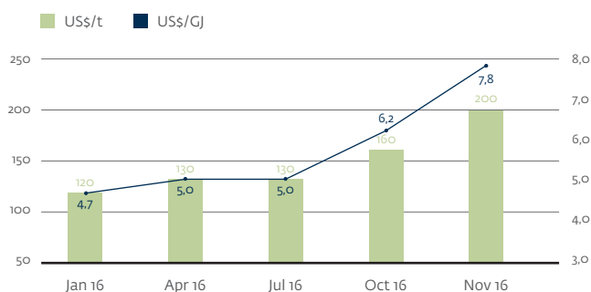
FIGURE 10. COAL PRICE TREND IN ETHIOPIA
