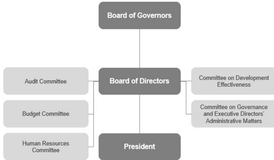
Figure 29: Governance Structure
