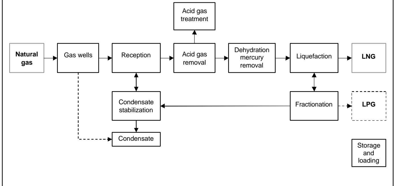
Figure A.1: Liquefied Natural Gas Production
